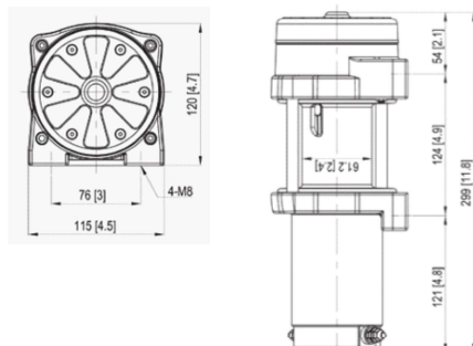
GTD2200 (12v/24v) – mm/in
