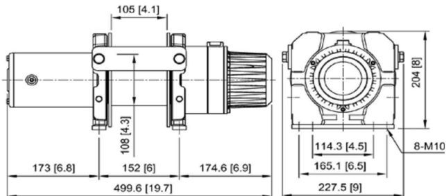
GTD2200 (12v/24v) – mm/in
