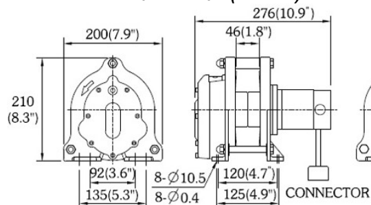
DH120 / DH120A (12v/24v) – mm/in
