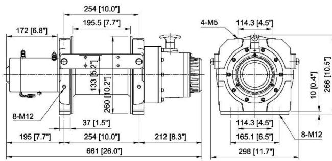
Rhino 15 (24V DC) – mm/in
