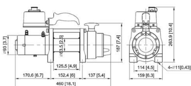
DV-6S 12V mm/in
