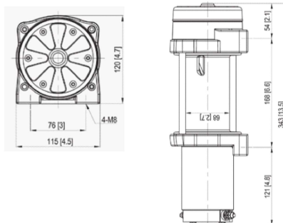
GTD800 (12v/24v) – mm/in
